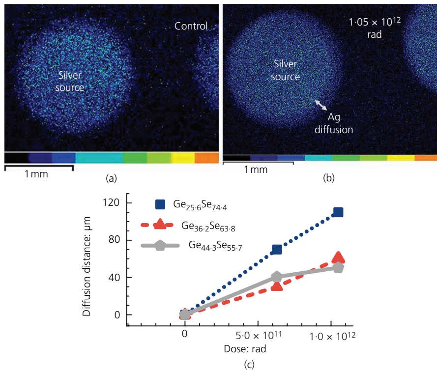
Figure 6. EDS mapping data of silver diffusion distribution in \text{Ge}_{25.6}\text{Se}_{74.4} exposed to (a) 0 and (b) 1.05 \times 10^{12} rad; (c) total diffusion distance as determined from mapping data for three compositions
