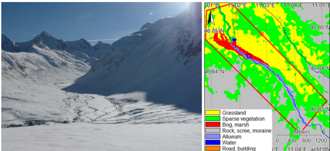
Figure 9. Photograph (20 November 2012) and land cover map of the Rotmoos valley with approximate area covered by SnowSAR indicated within the red line. Location of weather station indicated by purple dot.
